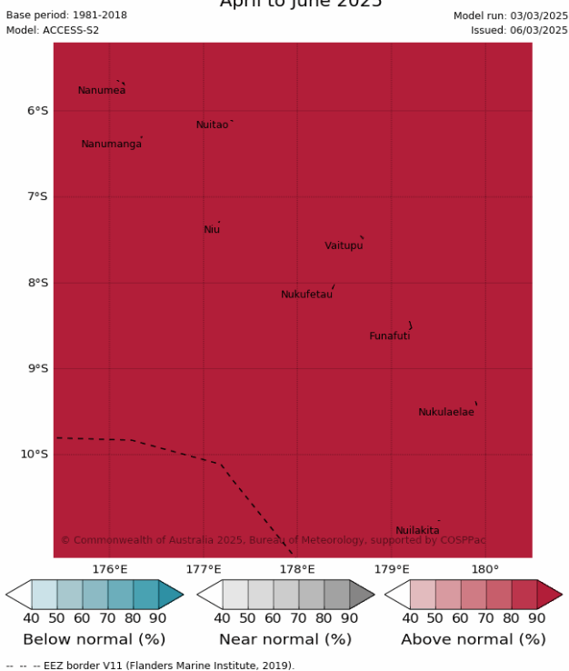
Tercile maximum temperature probabilities for April to June 2025
