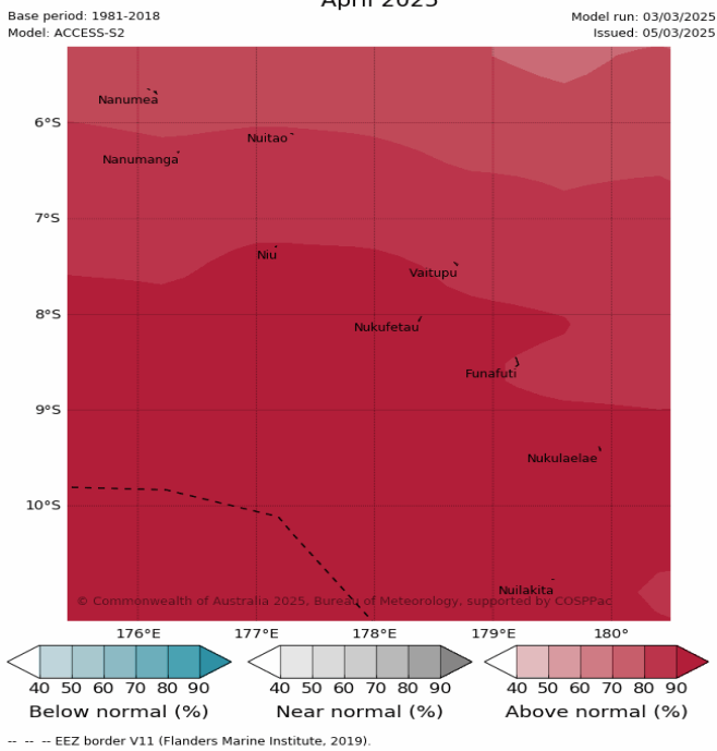
Tercile minimum temperature probabilities for April 2025
