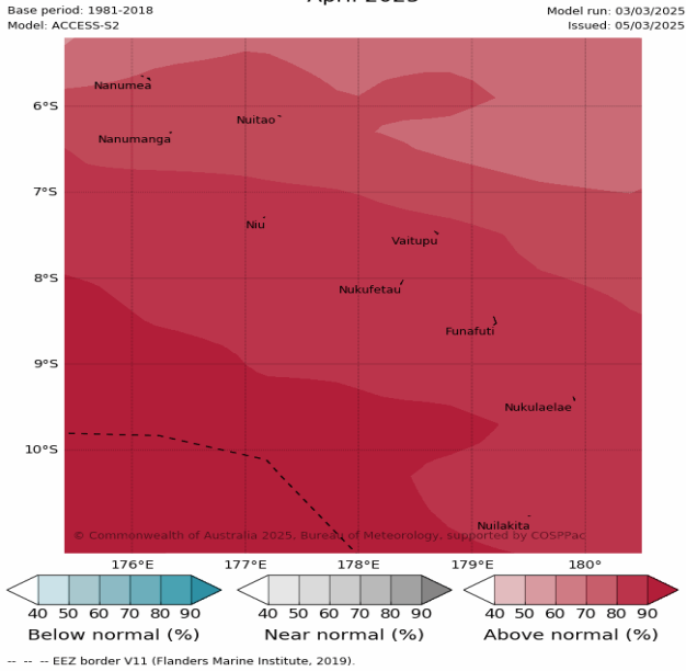
Tercile maximum temperature probabilities for April 2025
