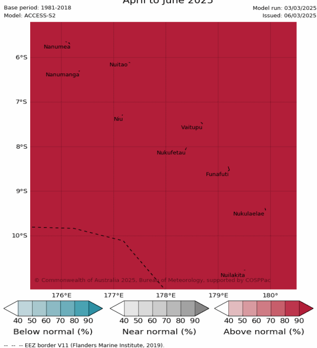
Tercile minimum temperature probabilities for April to June 2025
