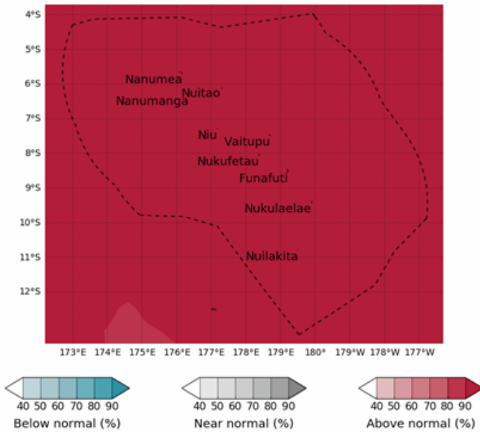
Tercile minimum temperature probabilities for July 2024
